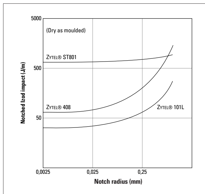
Figure 3.50 Effect of notch radius on Izod impact strength
