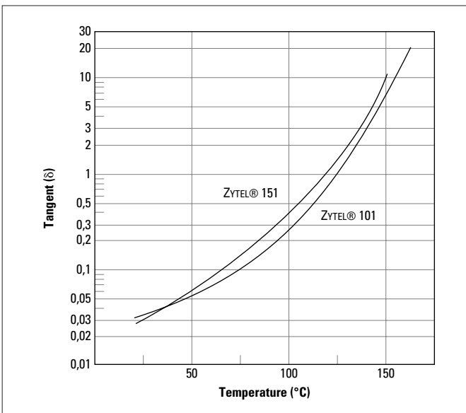
Figure 4.06 Dissipation factor vs. temperature (100 Hz). Samples conditioned to 50% RH at 23°C. Typical values based on laboratory measurements
