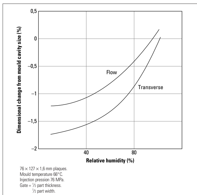
Figure 6.14 Dimensional changes in parts of ZYTEL® 408
