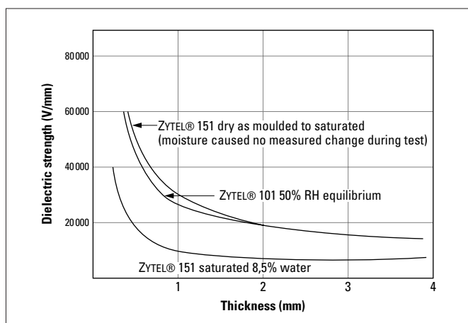
Figure 4.01 Short time dielectric strength of ZYTEL® vs. thickness measured at 23°C
