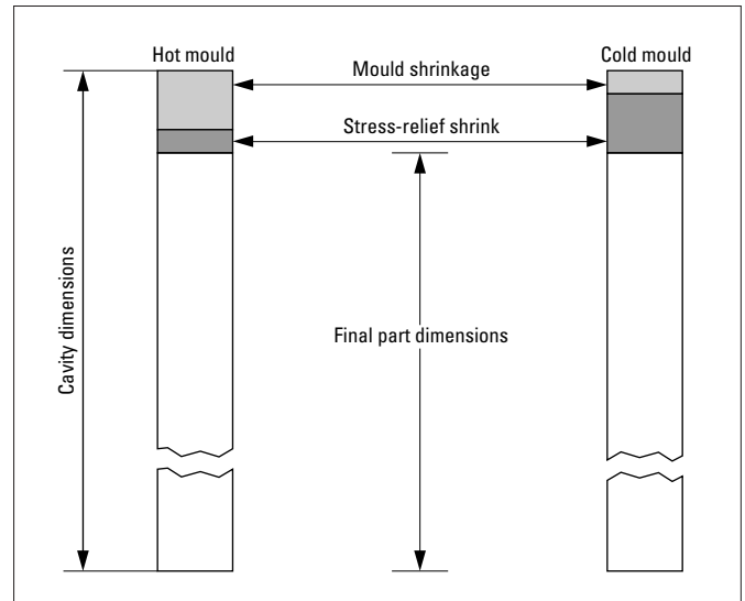
Figure 6.10 Effect of mould temperature on shrinkage dimensions
